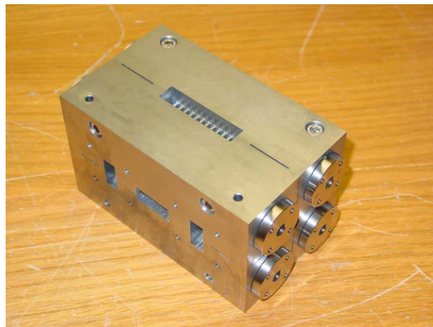
Figure 1: Photo of the assembled accelerating structure (HDX11mo) made out of 4 Molybdenum quadrants. Visible are the input and output coupler waveguides as well as the flanges to connect the water cooling pipes.
