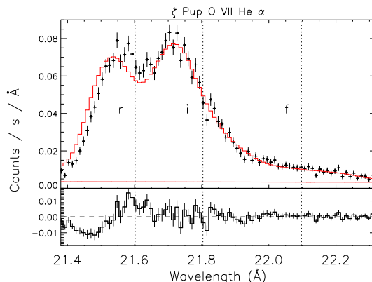
Figure 2: Same as Fig. 1, but for O VII.
