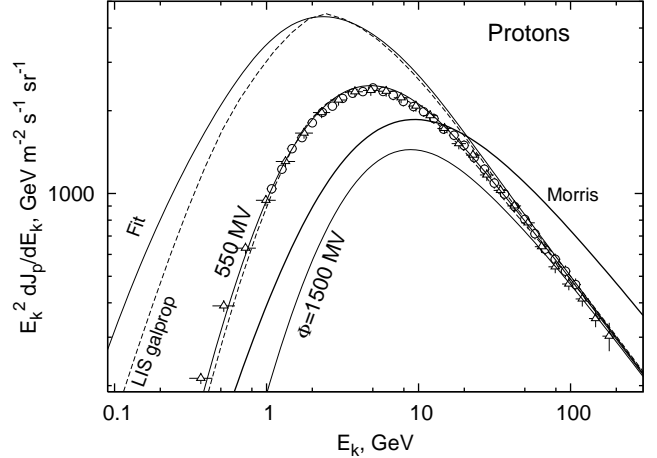
FIG. 3.— The CR proton spectrum. The dashed lines are the LIS spectrum (upper) and modulated one (lower, \Phi = 550 MV) as calculated by GALPROP in the plain diffusion model 44_999726 (Ptuskin et al. 2006). The thin solid lines are the fit to the LIS spectrum (upper) and modulated spectra (middle, \Phi = 550 MV; lower \Phi = 1500 MV). The thick solid line is the CR proton spectrum used by Morris (1984). Data: circles — BESS (Sanuki et al. 2000), triangles — AMS (Alcaraz et al. 2000a).
