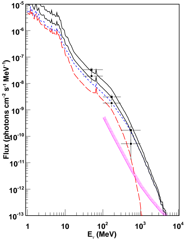
FIG. 4.— Calculated \gamma -ray albedo spectrum of the Moon. Line-styles: black-solid, total; blue-dotted, limb – outer 5' ; red-dashed, center – inner 20' . Upper solid line: \Phi = 500 MV; lower solid line: \Phi = 1500 MV. Limb and center components are only shown for \Phi = 1500 MV. Data points from the EGRET (Thompson et al. 1997) with upper and lower symbols corresponding to periods of lower and higher solar activity, respectively. The differential 1 year sensitivity of the LAT is shown as the shaded region.
