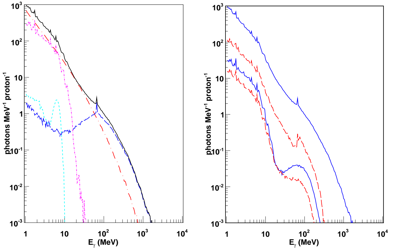
FIG. 2.— \gamma -ray yield per proton interaction integrated over all emission angles from the Moon surface. Left panel: yield calculated for E_p = 10000 MeV and \cos \theta_p = 0.1 with components shown. Line styles: blue-dashed, decay; red-long-dash-dot, bremsstrahlung; magenta-short-dash-dot, non-elastic scattering and de-excitation; cyan-dot, low energy neutron capture; black-solid, total. For each component, the initial process responsible for the production of the \gamma -ray secondary is given by the line style but the yield distribution includes also processes such as Compton scattering. Right panel: yield calculated for two different energies and incident angles. Line styles: blue-solid, \cos \theta_p = 0.1 ; red-dashed, \cos \theta_p = 1 . Line-sets: lower, E_p = 500 MeV; upper, E_p = 10000 MeV.
