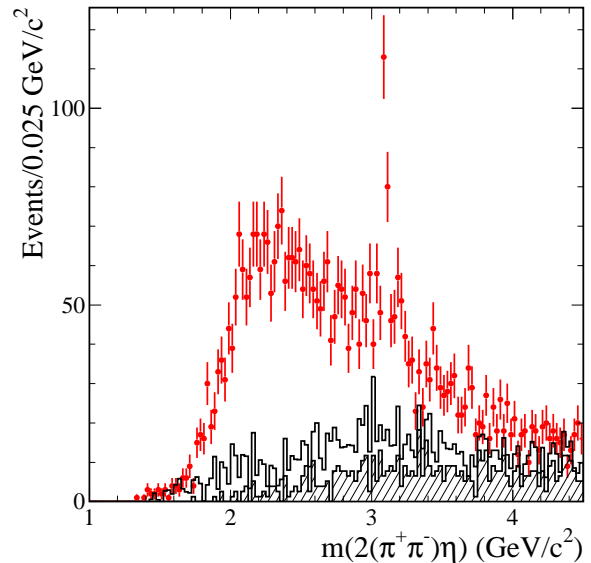
FIG. 21: Invariant mass distribution for selected 2(\pi^+\pi^-)\eta events in the data (points). The hatched and open histograms represent, cumulatively, the non-ISR background and the background from the control region of Fig. 20.
