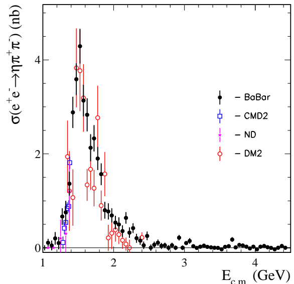
FIG. 11: The e^+e^- \rightarrow \eta\pi^+\pi^- cross section as a function of c.m. energy obtained via ISR at BABAR . The direct measurements from DM2, ND and CMD2 are also shown. Only statistical errors are shown.
