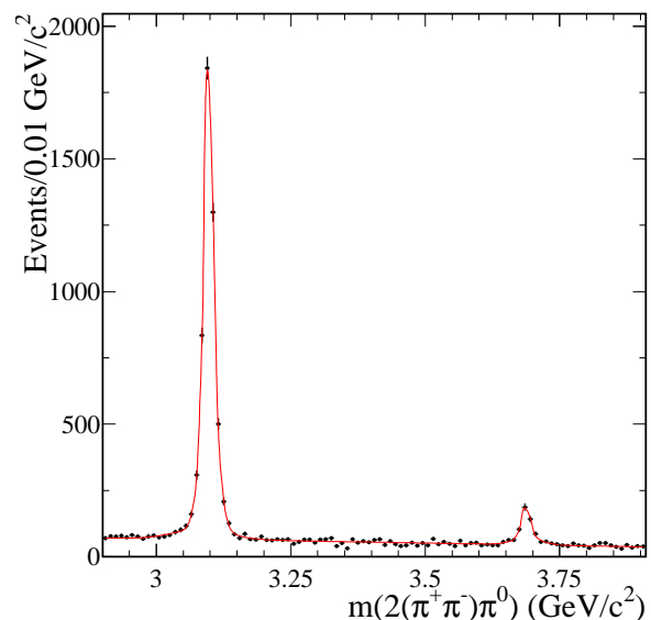
FIG. 38: Raw invariant mass distribution for all selected e^+e^- \rightarrow 2(\pi^+\pi^-)\pi^0 events in the charmonium region. The line represents the result of the fit described in the text.
