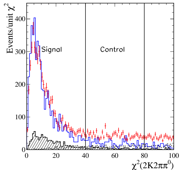
FIG. 26: Distribution of \chi^2 from the 5C fit for K^+K^-\pi^+\pi^-\pi^0 candidates in the data (points). The open histogram is the distribution for simulated signal events, normalized as described in the text. The hatched and dashed histograms are the backgrounds from non-ISR events and ISR K^+K^-\pi^+\pi^-\pi^0 events, respectively, estimated as described in the text
