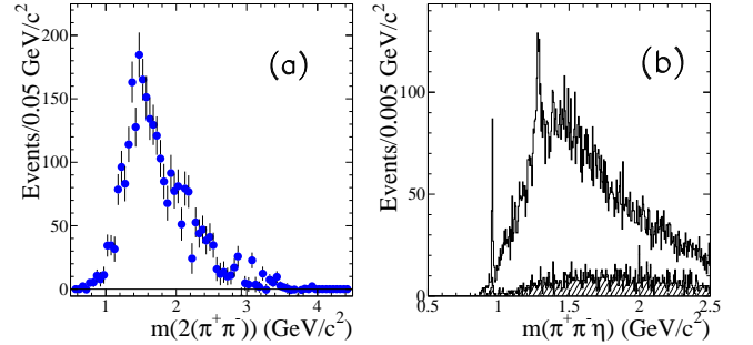
FIG. 23: (a) Background-subtracted invariant mass distribution for the four pions recoiling against the \eta in 2(\pi^+\pi^-)\eta events. (b) Invariant mass distribution for all \pi^+\pi^-\eta combination (four entries per event) in selected 2(\pi^+\pi^-)\eta candidates (open histogram) and the estimated non-ISR background (hatched).
