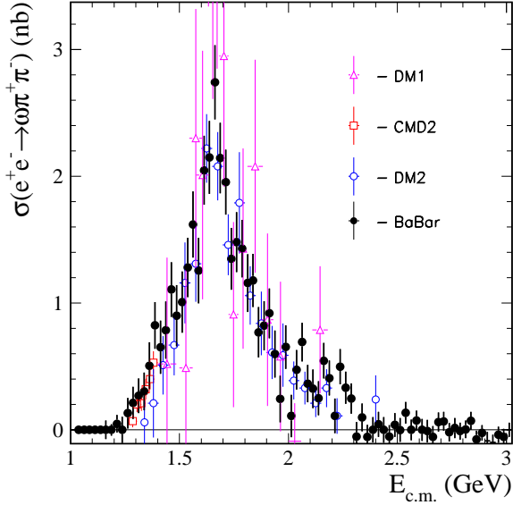
FIG. 14: The e^+e^- \rightarrow \omega\pi^+\pi^- cross section as a function of c.m. energy obtained via ISR at BABAR . The direct measurements from DM1, DM2 and CMD2 are also shown. Only statistical errors are shown.
