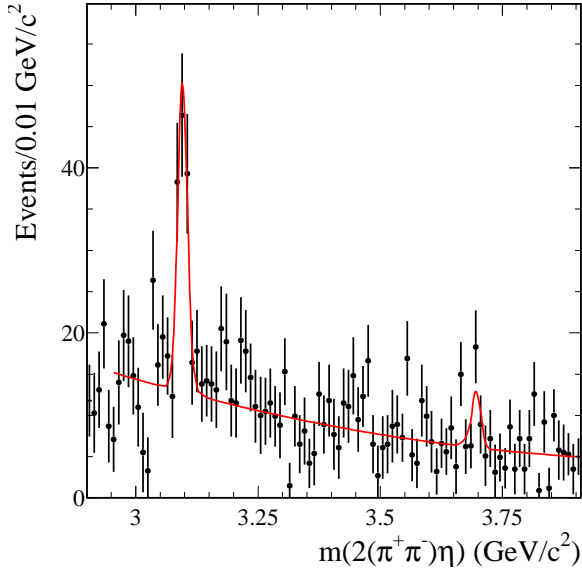
FIG. 39: Raw invariant mass distribution for all selected e^+e^- \rightarrow 2(\pi^+\pi^-)\eta events in the charmonium region. The line represents the result of the fit described in the text.
