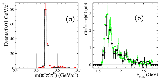
FIG. 32: (a) The \pi^+\pi^-\pi^0 mass distribution in the region below 700 MeV/c 2 for events with a K^+K^- mass within 15 MeV/c 2 of the \phi mass (points). The histogram is the distribution for the ISR \phi\eta simulation. (b) The e^+e^- \rightarrow \phi\eta cross section measured here in the K^+K^-\pi^+\pi^-\pi^0 final state (large dots), compared with the previous BABAR measurement in the ISR K^+K^-\gamma\gamma final state [27].
