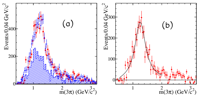
FIG. 18: (a) The invariant mass distributions for \pi^+\pi^-\pi^0 (triangles) and \pi^+\pi^-\pi^\pm (squares) combinations for events in which the other \pi^+\pi^- or \pi^\pm\pi^0 pair is in the \rho signal region. The hatched histogram is an estimate of the combinatorial background. (b) The average of the triangles and squares in (a) minus the combinatorial background. The line is the result of a Breit-Wigner fit.
