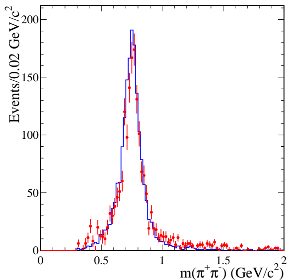
FIG. 9: Invariant mass distribution of the \pi^+\pi^- pair not from the \eta in selected \eta\pi^+\pi^- events in the data (points) and in simulated \eta\rho events (histogram).
