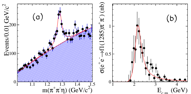
FIG. 25: (a) Distribution of the \pi^+\pi^-\eta invariant mass in the 1\text{--}1.5 \text{ GeV}/c^2 region for the data (points). The line represents the result of the fit described in the text, with the shaded region representing the background component. (b) The e^+e^- \rightarrow f_1(1285)\pi^+\pi^- cross section obtained via ISR. The line is the result of the Breit-Wigner fit described in the text.
