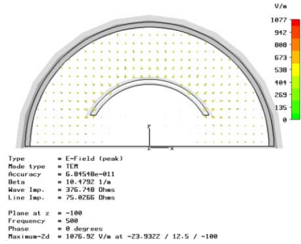
Figure 3: Microwave Studio output for the even TEM mode.
