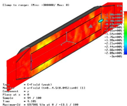
Figure 6: Electric field map at the time the trailing bunch enters the kicker structure.
