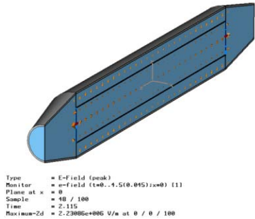
Figure 5: Example of time frame of the electric field on the kicker vertical mid-plane.
