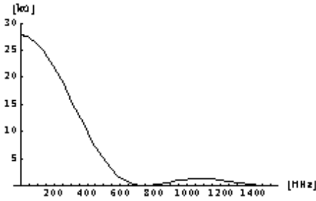
Figure1: Kicker shunt impedance.
