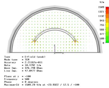
Figure 2: Microwave Studio output for the odd (kicking) TEM mode.
