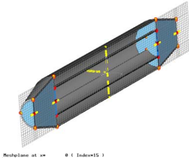
Figure 4: 3D mesh of the kicker with tapers.
