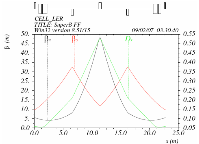
Figure 4 LER arc lattice cell.
