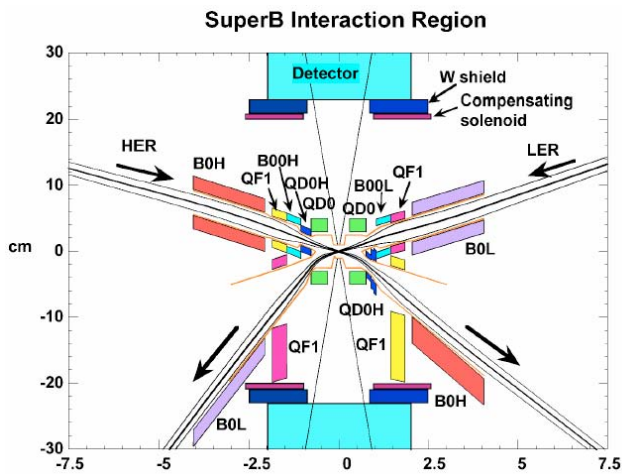
Figure 3 Interaction region for two asymmetric beams.
