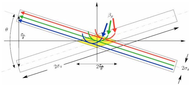
Figure 2 Interaction region showing two thin beams crossing at a large angle with crab waist to improve the beam-beam interaction.
