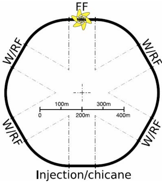
Figure 1 Super-B Factory with circumference = 2250 m.
