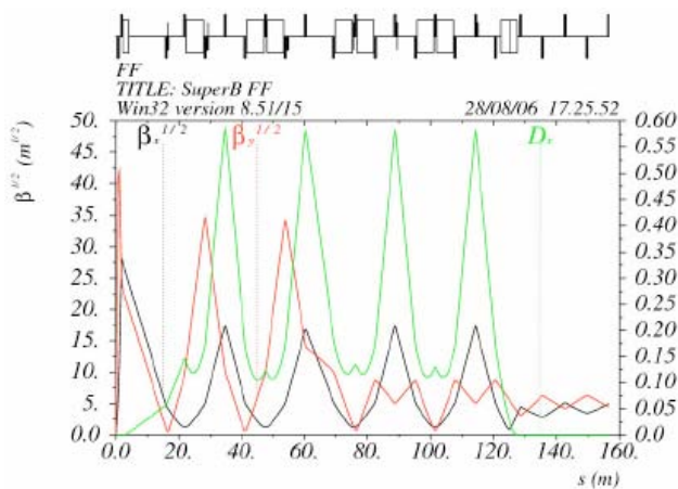
Figure 5 IR optical parameters for a Super-B-Factory.
