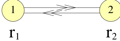
Figure 1: Quiver diagram for the conifold singularity. Each node is an SU(r_i) gauge group, and each arrow is a bifundamental field. The difference in ranks counts the number of fractional D5-branes.
