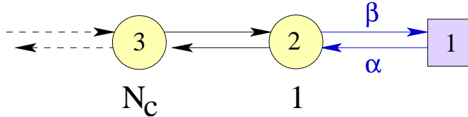
Figure 6: The extended quiver diagram, including a node for the Euclidean D-brane.
