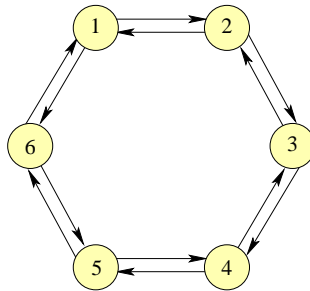
Figure 2: The quiver diagram of the orbifolded model for n = 3 .
