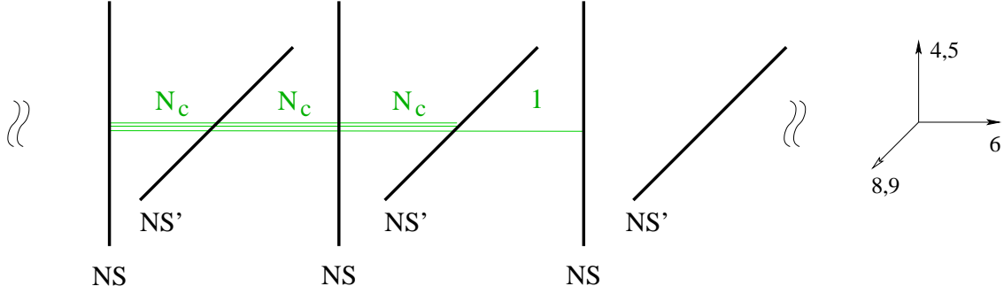
Figure 4: Type IIA T-dual description of the type IIB quiver in Figure 3.
