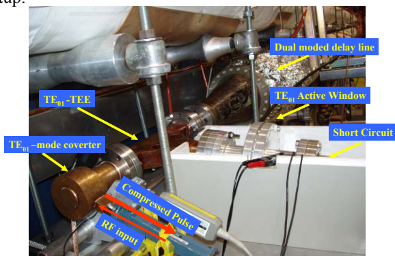
Figure 4: Active Pulse Compression Experiment Setup
