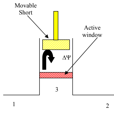
Figure 1: The tunable switch module.
