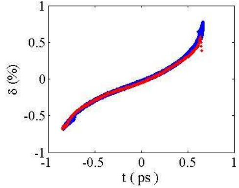
Figure 4: (color) The simulated measurement of the electron beam longitudinal phase space (using Eq.(6), red dots) and the ELEGANT simulation result (blue dots).
