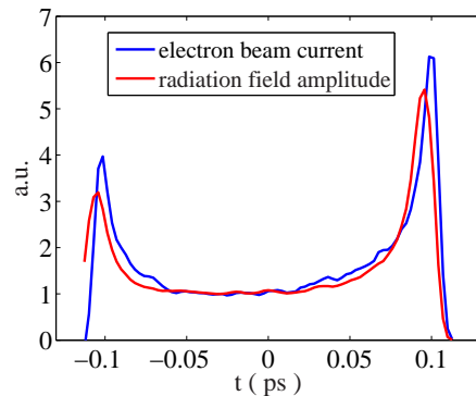
Figure 2: (color) The radiation field amplitude from the radiator and the electron current profile for the LCLS 1 nC case, bunch head at left.
