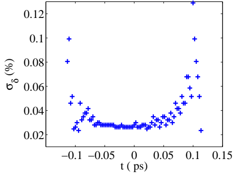
Figure 3: (color) The slice energy spread obtained from Eq.(3) by scanning R_{56} , bunch head at left.
