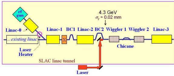
Figure 1: (color) Schematic of the OR setup at LCLS
