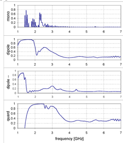
Figure 6: Absorbing parameters of a new Q2 absorber
