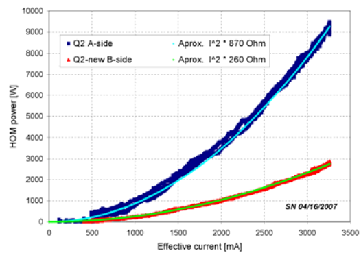
Figure 9: HOM power in one old and one new Q2-bellows.
