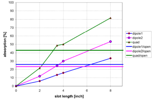
Figure 4: Absorption vs slot length and absorption levels of exposed tiles.
