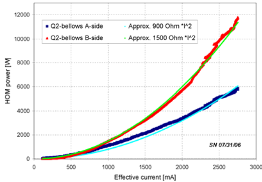
Figure 2: HOM power in the “old” Q2-bellows. LER rf voltage is 4.05 MV, HER rf voltage is 15.4 MV, number of bunches is 1722.
