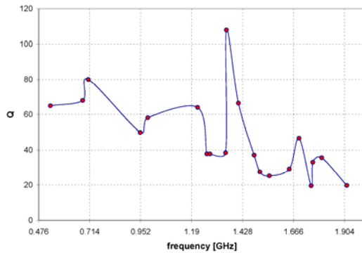
Figure 7: Q-values of HOMs trapped inside bellows cavity. Dotted vertical lines depict bunch spacing frequencies.
