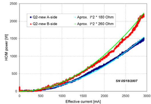
Figure 10: HOM power in all new Q2-bellows.
