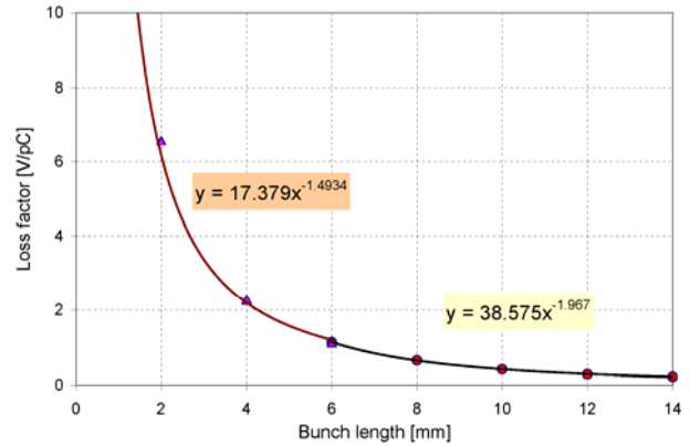
Figure 1: IP geometric loss factor vs bunch length.
