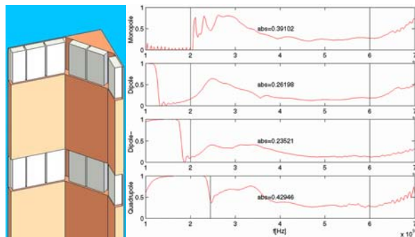
Figure 3: Computer model of the old Q2 (one quarter) and absorbing parameters.
