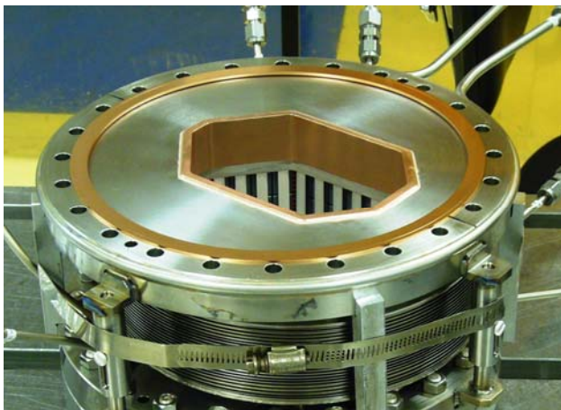
Figure 8: A new Q2-bellows absorber.
