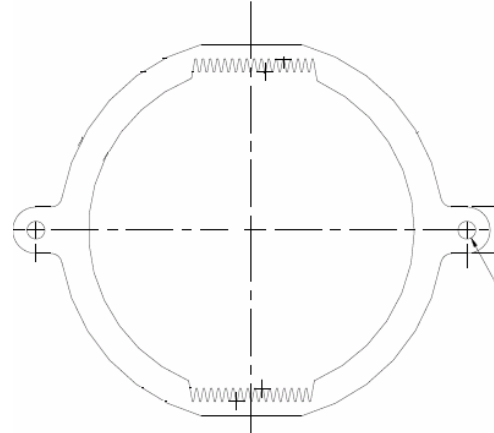
Figure 7: Sketch of the beam pipe with grooved surface in a dipole magnet
