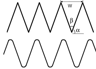
Figure 1 Triangular grooved surface: triangular surface with sharp tips (top) and triangular surface with rounded tips (bottom).
