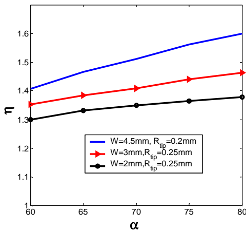
Figure 5: Impedance enhancement factor of the triangular grooved surface with round tips.
