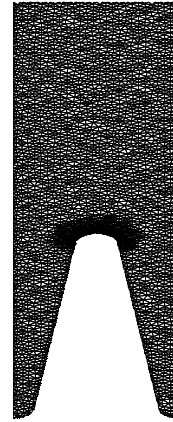
Figure 2: Adaptive mesh of the grooved surface.
