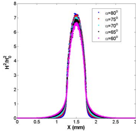
Figure 4: Magnetic fields on the grooved surface with rounded tip. A period of a groove is shown. The geometry of the surface is shown in Figure 2. The field is normalized by the field with flat surface. The peak field locates at the surface near the tip.
