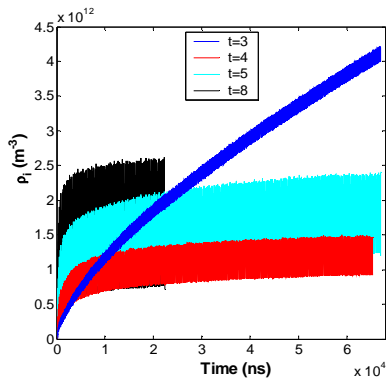
Figure 5: build-up of ion cloud with different emittance at different time after beam injection.
