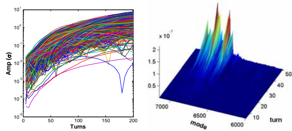
Figure 3: Simulated vertical oscillation amplitude and beam instability spectrum with realistic optics. The total number of bunches is 5782 and the pressure is 1 nTorr of CO+.
