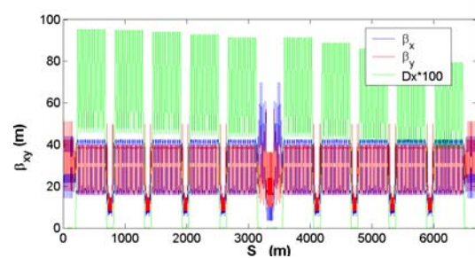
Figure 1: Optics of ILC 6km-damping ring
