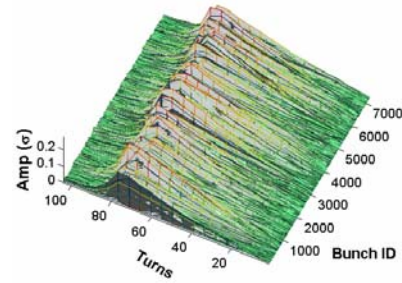
Figure 6: Damping of beam instability using bunch-by-bunch feedback. The total number of bunch is 5782.
