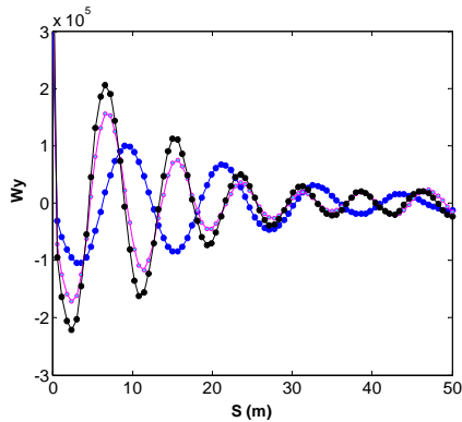
Figure 4: Vertical wake of the ion cloud for different bunch intensity
