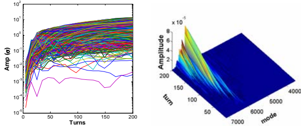
Figure 2: Simulated vertical oscillation amplitude and beam instability spectrum with one ion-beam interaction point. The total number of bunches is 5782. The pressure is 1 nTorr of CO+.
