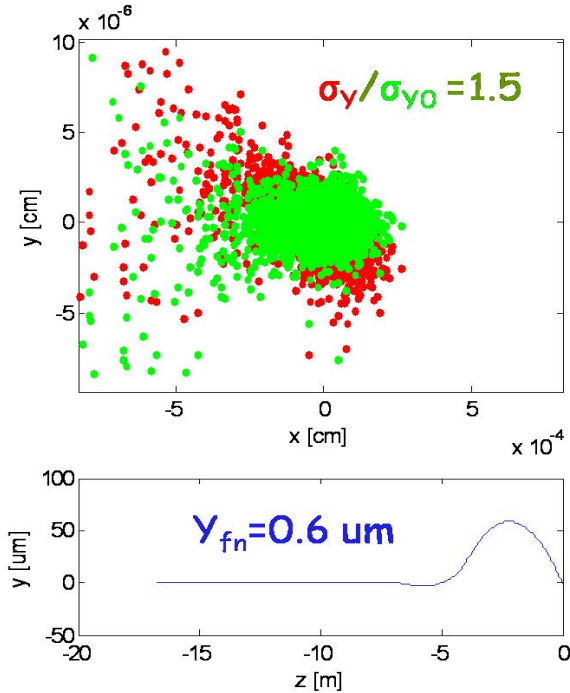
Figure 4: Beam profile (upper plot) and vertical projection of beam's trajectory (lower plot) in the IP for GLD solenoid field compensated with Weak Antisolenoid. Green dots in the upper plot represent nominal beam; red dots stand for the compensated beam. 1E4 particles were tracked.
