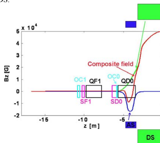
Figure 1: Final Doublet in the fields of the Detector Solenoid (green line) and the Weak Antisolenoid (blue line). The IP is at z=0 m. This plot is given for the length of the final drift L^*=3.51 m and a Silicon Detector (SiD) solenoid field.
