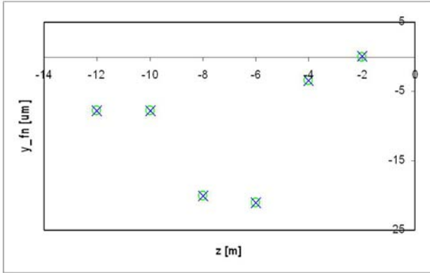
Figure 3: Vertical offset of beam trajectory in the IP depending on the position of test solenoid. Analytical results are presented by 'o'; simulations are shown by 'x'. Optics with L^*=3.51 m and \theta_s=10 mrad is chosen for this exercise.
