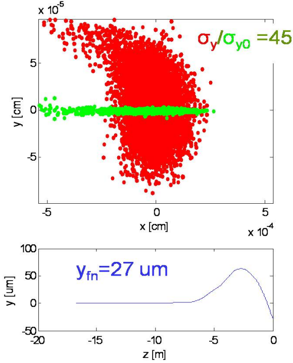
Figure 2: The effect of uncompensated DS field on the vertical beam size (upper plot) and beam trajectory in the IP (lower plot). The beam size ( \sigma_y ) is characterized by the “luminosity equivalent sigma” [5]. Green dots stand for the nominal beam profile; red dots show the uncompensated beam. These plots are given for GLD solenoid field and L^*=4.5 m.
