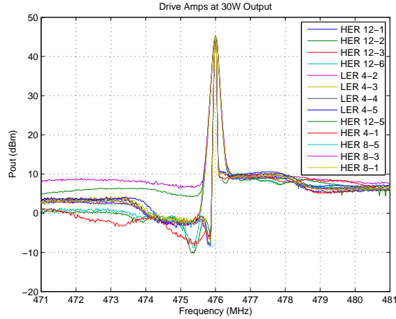
Figure 4: Swept Sideband Image responses for 12 Amplifiers "A"
