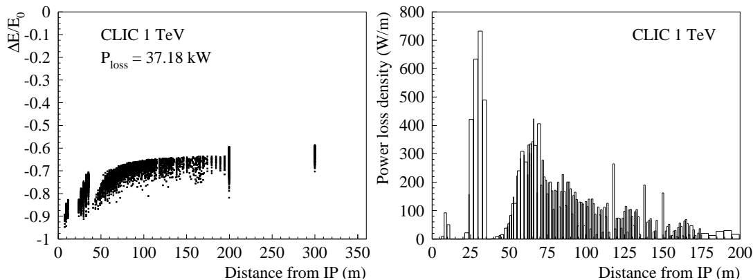
Figure 1: Relative energy spread of the lost particles as a function of the position of loss in the 20 mrad extraction line (left) and loss density upstream of the collimators (right), obtained when tracking the disrupted beam of the 1 TeV CLIC case.
