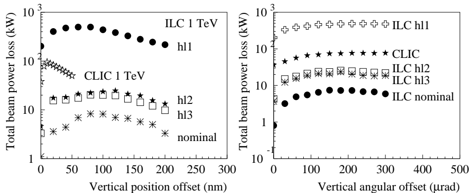
Figure 2: Disrupted beam power losses in the extraction line as a function of the position offset \Delta y (left) or the angular offset \Delta y' (right), for various ILC and CLIC configurations at 1 TeV.
