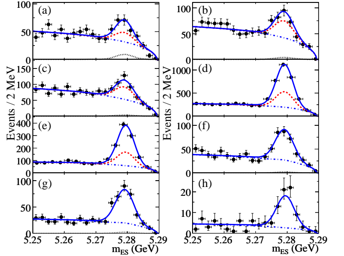
FIG. 2: Plots of signal-enhanced subsets of the data distributions projected onto m_{ES} for the decays: (a) B^+ \rightarrow \eta\pi^+ , (b) B^+ \rightarrow \eta K^+ , (c) B^+ \rightarrow \eta'\pi^+ , (d) B^+ \rightarrow \eta'K^+ , (e) B^0 \rightarrow \eta'K^0 , (f) B^+ \rightarrow \omega\pi^+ , (g) B^+ \rightarrow \omega K^+ , and (h) B^0 \rightarrow \omega K^0 . The solid line represents the result of the fit, and the dot-dashed line the background contribution. The dashed line gives the sum of background and the \eta_{3\pi} (a, b) or \eta'_{\eta\pi\pi} (c-e) component of the signal. The dotted line shows the K or \pi cross-feed component, where applicable.
