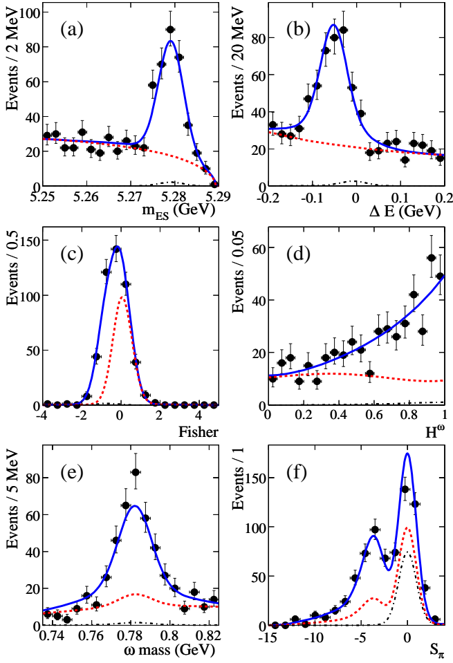
FIG. 1: Plots of signal-enhanced subsets of the data distribution for B^+ \rightarrow \omega K^+ projected on each of the fit variables: (a) m_{ES} , (b) \Delta E , (c) \mathcal{F} , (d) \mathcal{H}^\omega , (e) \omega mass, and (f) S_\pi . Points with errors represent the data, solid curves the full fit functions, dashed curves the sum of the background functions, and dot-dashed curves the signal from B^+ \rightarrow \omega\pi^+ . The variable \Delta E is computed with the pion mass.
