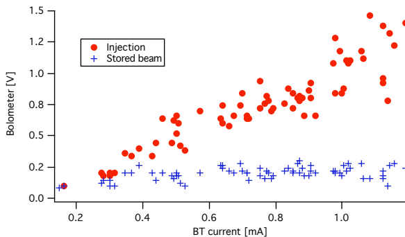
Figure 6: Bolometer signal from injection a stored beam as a function of the bunch current (injection transfer line current monitor).
