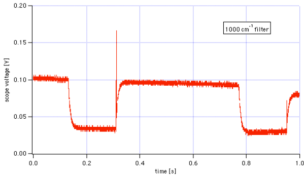
Figure 5: Typical bolometer signal ( 1000\text{ cm}^{-1} filter). Bunch is dumped 450 ms after injection. Injection period is 650 ms.
