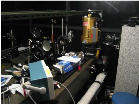
Figure 2: Experimental set-up at the ATF diagnostic beamline.
