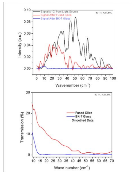
Figure 3: Experimental measurements of the attenuation in the near-infrared region from BK7 optical glass and water-free fused silica.
