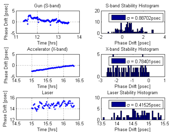
Figure 2: Phase measurement of the S-band in the gun, the X-band in the accelerator, and the laser sent to the photocathode. The y axis is phase between the reference and the signal of interest, and the x axis is time of the day in hours. The rms stability of each of the phases is shown in the histograms to the right.
