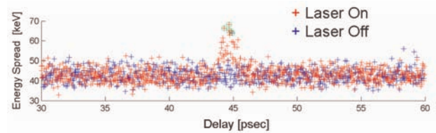
(a) Energy spread of electron beam
