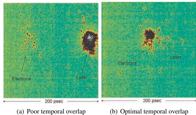
Figure 3: The path length in the laser transport line was adjusted until the faint image from the cherenkov radiation in 3(a) overlapped the clear image from the laser. The result is shown in 3(b). This allows for coarse timing overlap better 50 psec.
