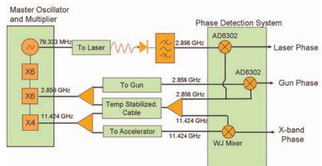
Figure 1: Schematic of the RF phase detection system implemented at the NLC Test Accelerator at SLAC.
