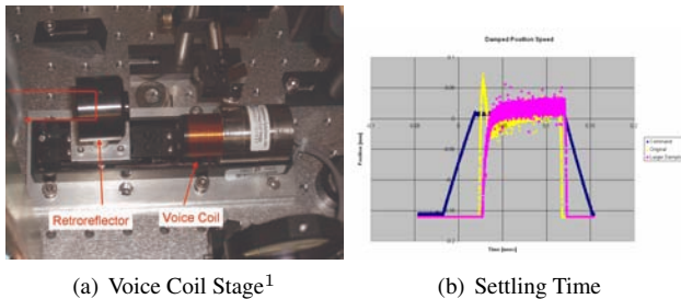
Figure 4: The voice coil controlled translation stage is used to adjust the laser transport path length at a 10 Hz rep rate, with an accuracy of 25\ \mu\text{m} (.083 psec), and a range of 30 mm (100 psec).
