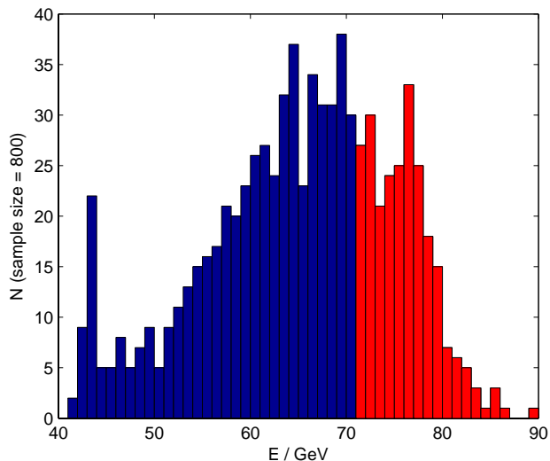
Figure 3: In 800 consecutive events, more than 30% showed an energy gain greater than 30 GeV. The plasma density was 2.7 \cdot 10^{23}/\text{m}^3 , the plasma length 85 cm.
