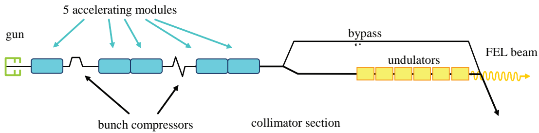
Figure 1: Schematic of the FLASH facility.
