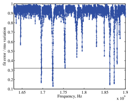
Figure 5: Dipole mode identification: Magnification of the area of the first and second dipole bands.
