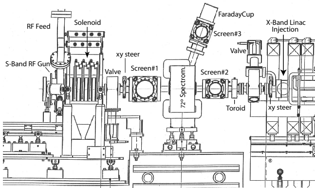
Figure 1: Layout of the SLAC NLCTA RF photoinjector.
