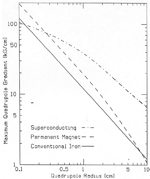
Figure 3: Strengths obtainable for different quads types[?]: iron pole-tip fields B_p=12 kG, remanent fields B_r=11.5 kG for PMs and NbTi wire with J_c=2 kA/mm 2 at 5T & 4.2°.
