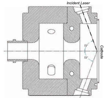
Figure 2: Schematic, cross-sectional view of a 1.6-cell, laser-driven RF gun. The internal, unshaded areas are to be maintained continuously at very high vacuum to sustain a stable and acceptable quantum efficiency as well as avoid RF breakdown damage. L or S-Band RF cells set the scale.
