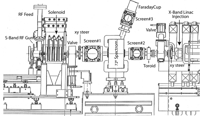
Figure 1: Layout of the SLAC E163 RF photoinjector line.
