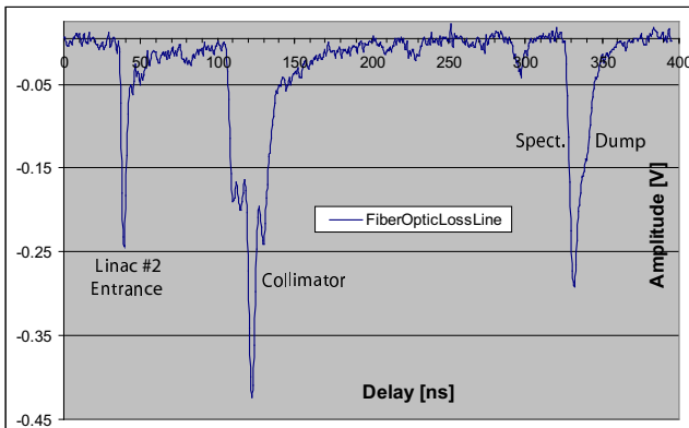
Figure 2: Trace of Fiber Optic Loss Line (FOLL) running from the NLCTA injector to the E163 spectrometer dump.
