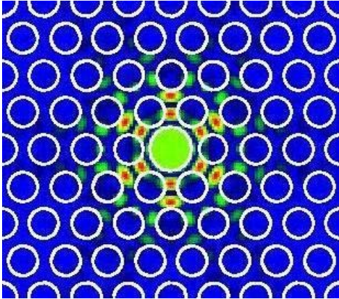
Figure 1: Accelerating field intensity of a 1 \mu\text{m} mode in a Lin fiber as calculated with CUDOS. The longitudinal direction is out of the page. The color scale is relative with red being the highest field and blue the lowest.
