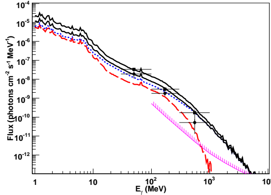
Figure 3: Calculated \gamma -ray albedo spectrum of the Moon. Line-styles: black-solid, total; blue-dotted, limb – outer 5' ; red-dashed, centre – inner 20' . Upper solid line: \Phi_0 = 500 MV; lower solid line: \Phi_0 = 1500 MV. Data points from the EGRET [11] with upper and lower symbols corresponding to periods of lower and higher solar activity, respectively. The differential 1 year sensitivity of the LAT is shown as the hatched region.
