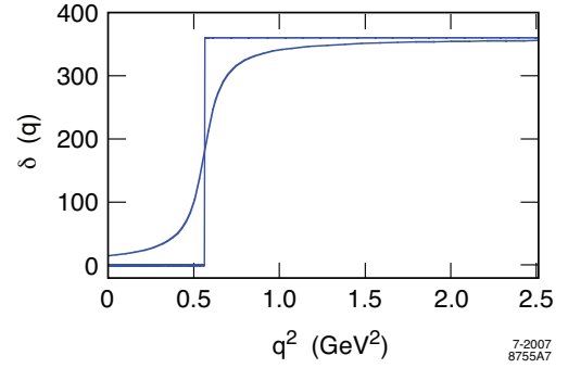
FIG. 6: Time-like pion form factor phase \delta_\pi(q) as a function of q^2 for \kappa = 0.375 GeV in the soft-wall model. The sharp curve corresponds to \Gamma = 0 and the smooth curve to \Gamma = 100 MeV.
