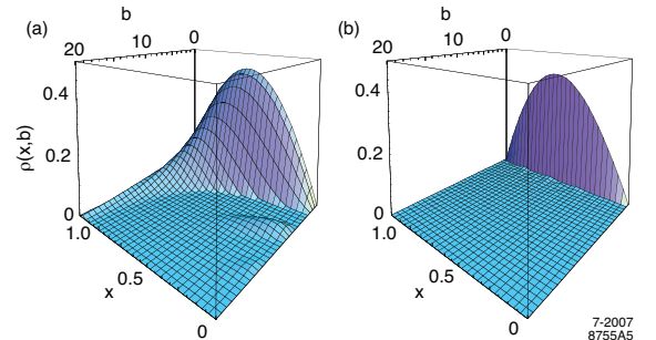
FIG. 7: Effective partonic density \rho(x, b, Q) in terms of the longitudinal momentum fraction x , the transverse relative impact variable b = |\mathbf{b}_\perp| and momentum transfer Q for the soft wall model. As Q increases the distribution becomes increasingly important near x = 1 and \mathbf{b}_\perp = 0 . This is illustrated in (a) for Q = 1 GeV/c. At very large Q (figure (b)), the distribution is peaked towards \mathbf{b}_\perp = 0 . The value of \kappa is 0.375 GeV.
