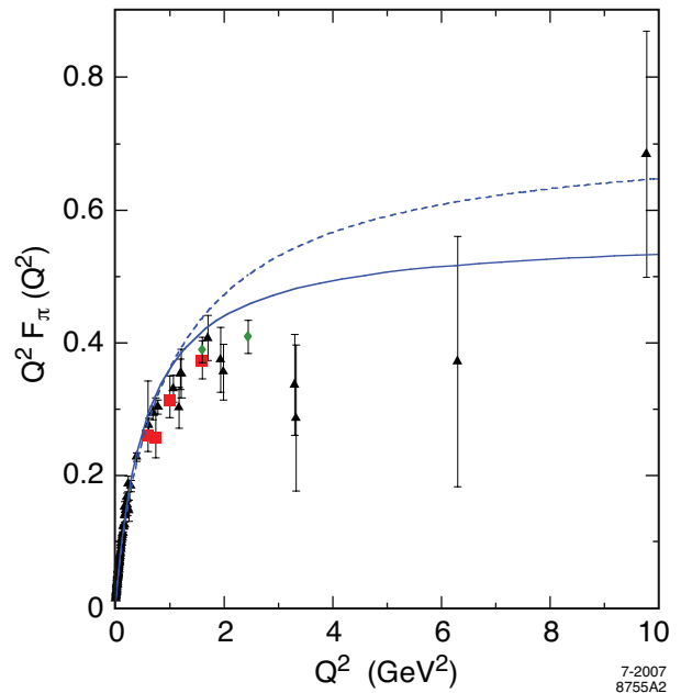
FIG. 2: Space-like scaling behavior for Q^2 F_\pi(Q^2) as a function of Q^2 = -q^2 . The continuous line is the prediction of the soft-wall model for \kappa = 0.375 GeV. The dashed line is the prediction of the hard-wall model for \Lambda_{QCD} = 0.22 GeV. The black triangles is the data compilation from Baldini et al. [77], the red boxes are JLAB 1 data [78] and cobalt green diamonds are JLAB 2 data [79].
