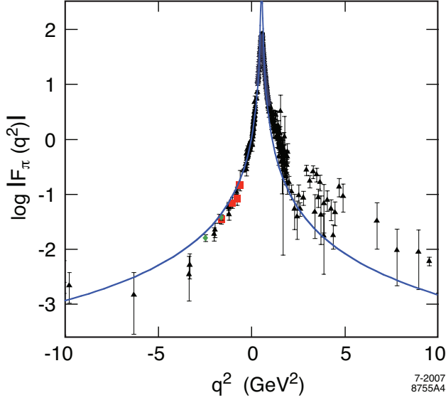
FIG. 4: Space and time-like behavior of the pion form factor \log(|F_\pi(q^2)|) as a function of q^2 for \kappa = 0.375 GeV in the soft-wall model. Black (triangle) is the data compilation from Baldini et al. [77], red (box) is JLAB 1 [78] and cobalt green diamonds are JLAB 2 [79].
