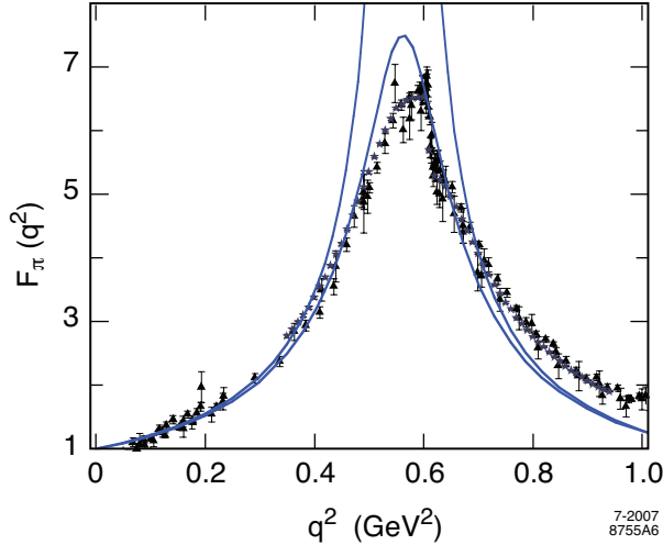
FIG. 5: Time-like pion form factor |F_\pi(q^2)| near the \rho peak as a function of q^2 for \kappa = 0.375 GeV in the soft-wall model. The upper curve correspond to \Gamma = 0 and the lower to \Gamma = 100 MeV. The data is from the compilation Baldini et al. [77].
