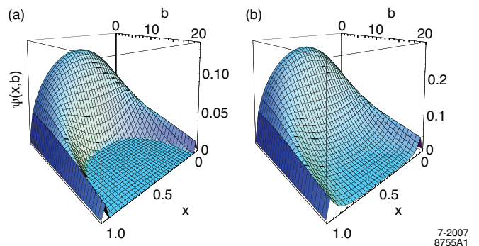
FIG. 1: AdS/QCD Predictions for the ground state light-front wavefunction of a pion in impact space. Left: truncated space model for \Lambda_{\text{QCD}} = 0.22 GeV. Right: soft wall model for \kappa = 0.375 GeV.
