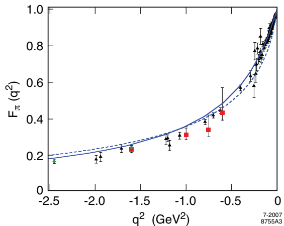
FIG. 3: Space-like behavior of the pion form factor F_\pi(q^2) as a function of q^2 for \kappa = 0.375 GeV and \Lambda_{QCD} = 0.22 GeV. Continuous line: soft-wall model, dashed line: hard-wall model. Black (triangle) is the data compilation from Baldini et al. [77], red (box) is JLAB 1 [78] and cobalt green diamonds are JLAB 2 [79].
