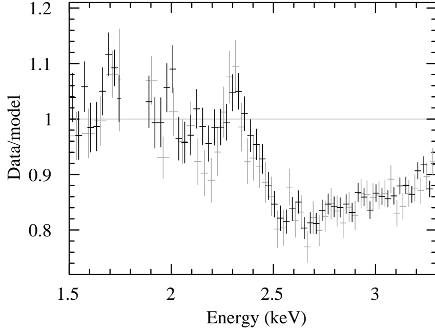
FIG. 8.— Residuals to a simple power-law model in the S K and Si K bandpass, showing the Si K\alpha emission line at 1.71 \pm 0.01 keV, the S K\alpha line at 2.307 \pm 0.016 keV, and the S K edge. Black points denote the three FI XIS spectra, which have been co-added for clarity; gray points denote XIS1. Rest-frame energies are shown. All data have been plotted with a binning factor of 10.
