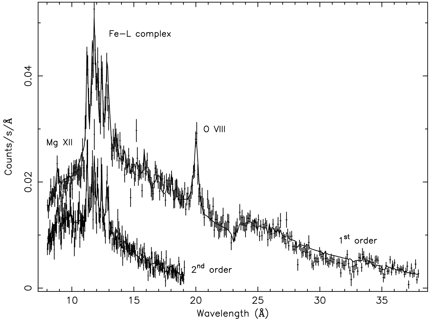
Fig. 5. 1^{\text{st}} and 2^{\text{nd}} order RGS spectrum of Sérsic 159-03 extracted from a 4' wide strip centred on the core. The continuous line represents the fitted wdem model. On the x-axis we show the observed wavelength.
