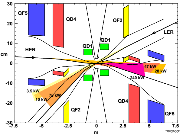
Figure 4: Interaction region for a Super B-Factor. The first quadrupole is at 35 cm from the interaction point.
