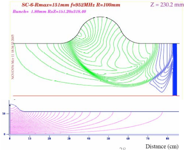
Figure 1: HOM calculation for a 952 MHz SC RF cavity with a 100 mm bore and RF fields along the beam line.
