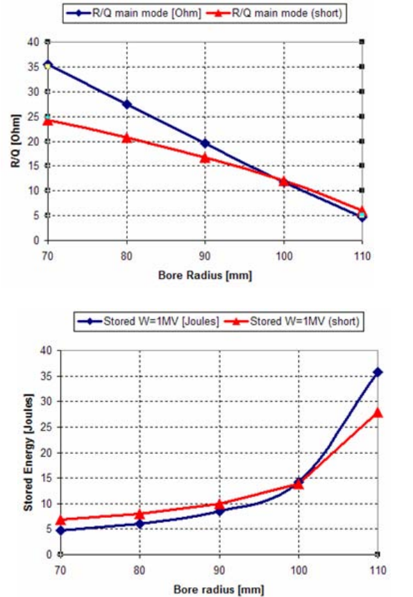
Figure 5: R/Q and stored field energy versus cavity bore.
