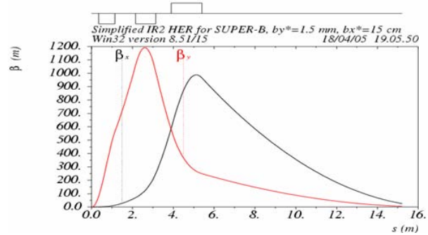
Figure 3: Beta functions in the HER interaction region.
