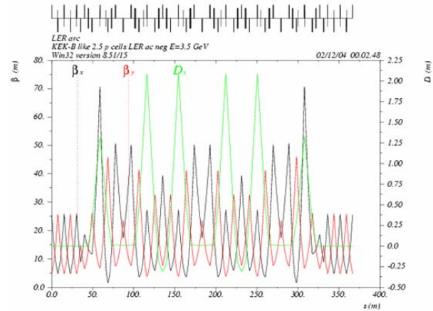
Figure 2: LER lattice with 2.5 \pi phase advance/cell.
