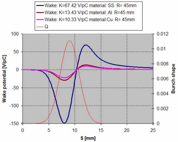
Figure 6: Resistive wall wakes for a 1.8 mm long bunch.
