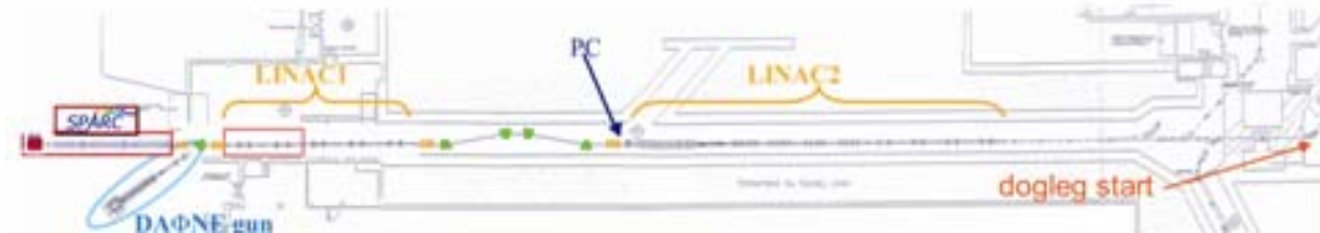
Figure 4: SPARXINO proposed layout.
