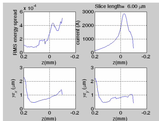
Figure 8: Energy spread, peak current and transverse emittance along the bunch, with the X-band ON at the magnetic chicane entrance.
