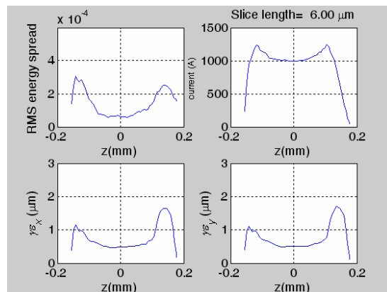
Figure 7: Energy spread, peak current and transverse emittance along the bunch, with the X-band ON at the RF gun exit.
