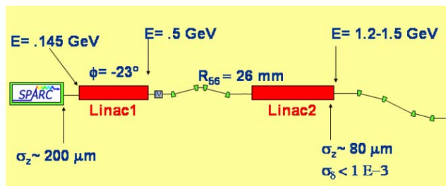
Figure 5: Schematic layout of the RF+magnetic compression scheme.
