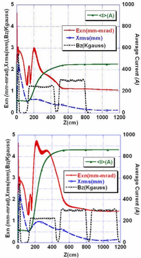
Figure 3: Peak current, normalized projected emittance, beam envelope and solenoid field map for two RF compressor working points.
