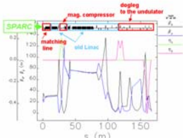
Figure 6: The SPARXINO lattice.
