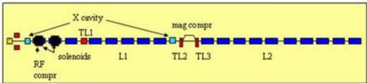
Figure 1: Schematic layout of the SPARXINO test facility.
