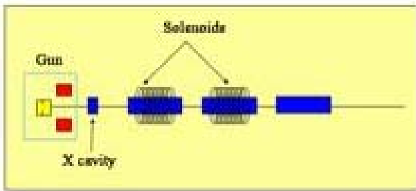
Figure 2: Schematic layout of the SPARXINO photoinjector.
