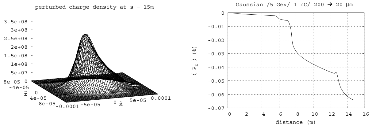
Figure 2: Left: Perturbed charge density at s = 15\text{m} (end of chicane). Right: Mean of the relative energy loss.
