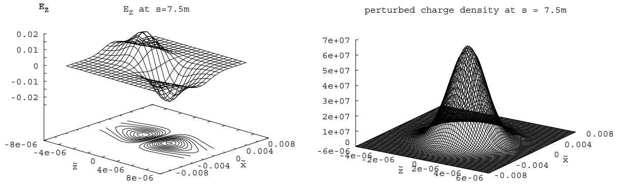
Figure 1: Left: E_Z at s = 7.5\text{m} (end of 3 rd magnet of the chicane). Right: Perturbed charge density at s = 7.5\text{m} .
