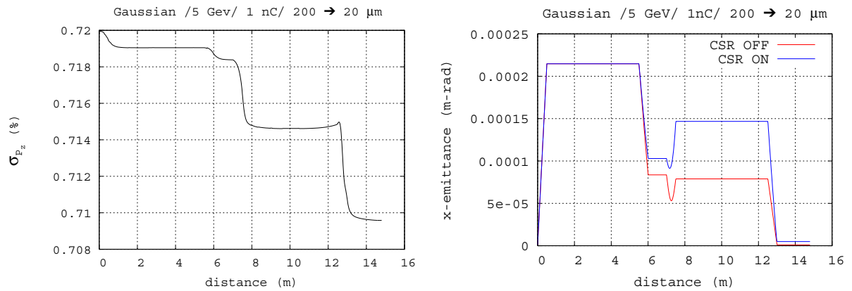
Figure 3: Left: Standard deviation of the relative energy deviation. Right: Normalized transverse emittance (x-emittance).
