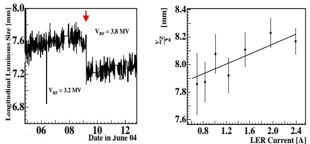
Figure 3: Left: history of the r.m.s. luminous length \sigma_z^L , before and after the LER RF voltage V_{RF}^+ was increased (arrow). The HER RF voltage V_{RF}^- remained constant. Right: e^+ -current dependence of the fitted value of \Sigma_z^L/2 ( \approx \sigma_z^L ) measured during a long coast-down. The line shows the fitted current-dependence (see text). The HER bunch length and the \beta functions are fixed in the fit.
