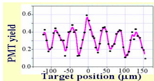
Figure 4: Radiation intensity image in detector plane measured using photo-multiplier.
