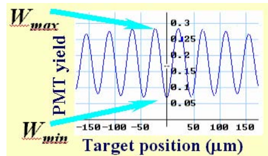
Figure 6: Calculated dependence of the radiation yield as a function of the vertical target position.
