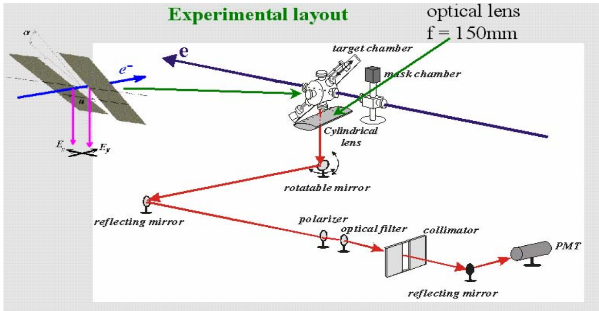
Figure 7: Principal scheme of experimental layout.
