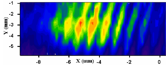
Figure 5: Measured dependence of the radiation yield as a function of the vertical target position.
