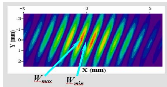
Figure 2: Theoretical radiation intensity image in detector plane for experimental conditions.
