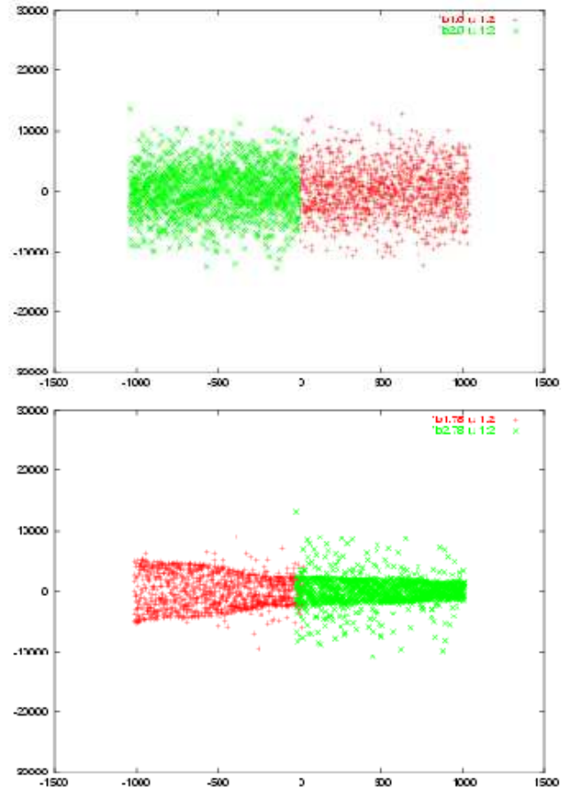
FIG. 20: Beams before (top) and after (bottom) collision: horizontal vs longitudinal ( z ) distribution. LER particles are red, HER particles are green.
