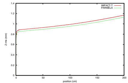
Figure 3: Longitudinal rms size as a function of distance.
