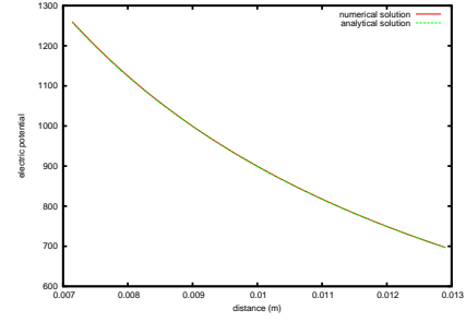
Figure 1: Image charge potential on the axis for a round beam from the shifted Green function solution together with the analytical solution.
