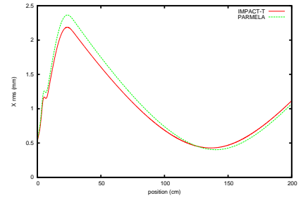
Figure 2: Transverse rms size as a function of distance.
