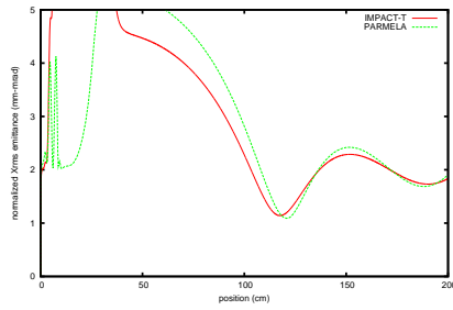
Figure 4: Transverse normalized rms emittance as a function of distance.
