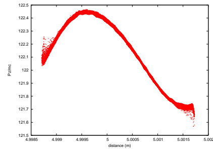
Figure 7: Longitudinal phase space distribution after the first traveling wave linac.
