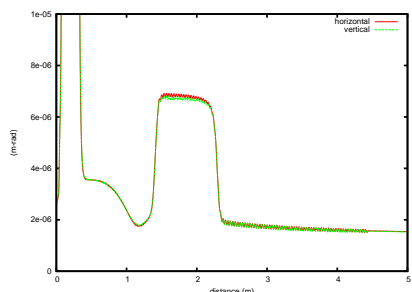
Figure 6: Transverse normalized rms emittance as a function of distance.
