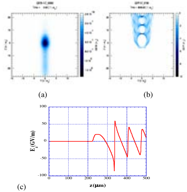
Figure 2. E164X simulation (a) Beam density at z=0 ; (b) Plasma density at z=8.6cm ; and (c) E_z at z=8.6cm .
