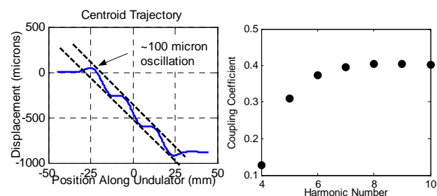
Figure 1: a) Centroid trajectory of electron bunch through undulator. b) Coupling coefficients from eq 2.
