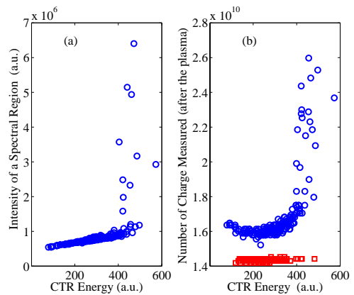
Figure 3: a) Relative amount of light recorded over a spectral region with no atomic lines as seen on Fig. 2. (b) Charge measured by a fast current monitor located after the plasma versus CTR energy,
