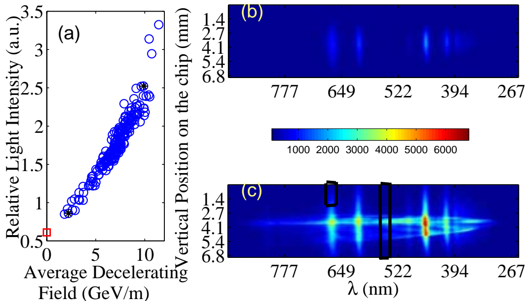
Figure 2: a) Intensity of the lithium atomic line at 670.8 nm, which is obtained from the sum of intensity counts inside the little box on trapped particle light free region on c, as a function of the average energy loss. The plasma density is constant at 1.6 \times 10^{17} \text{ cm}^{-3} (blue circles), the red square corresponds to plasma off events, and the energy loss varies because the bunch length varies from bunch to bunch. The line intensity is proportional to the mean beam energy, i.e., to the beam energy lost to the plasma wake. Lower marked circle indicate the event of b and upper marked circle indicate the event of c. b) Spectrograph image when there is no trapping corresponding to a relatively weak wakefield amplitude; c) image with trapping for a high wakefield amplitude. Light is a combination of discrete neutral line emission from the plasma, and continuum light from Cherenkov radiation in the gases and continuous OTR radiation at the mirror by relativistic beam and trapped particles (Note that the OTR light by the beam particles only is too weak to be visible on Fig. 2b)
