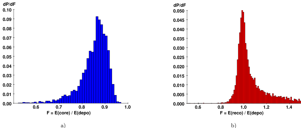
Figure 2: Part a) shows the fraction of energy from isolated photons reconstructed in the identified shower core. Part b) shows the fraction of energy reconstructed in refined showers for photons from K_s^0 \rightarrow \pi^0 \pi^0 decays.
