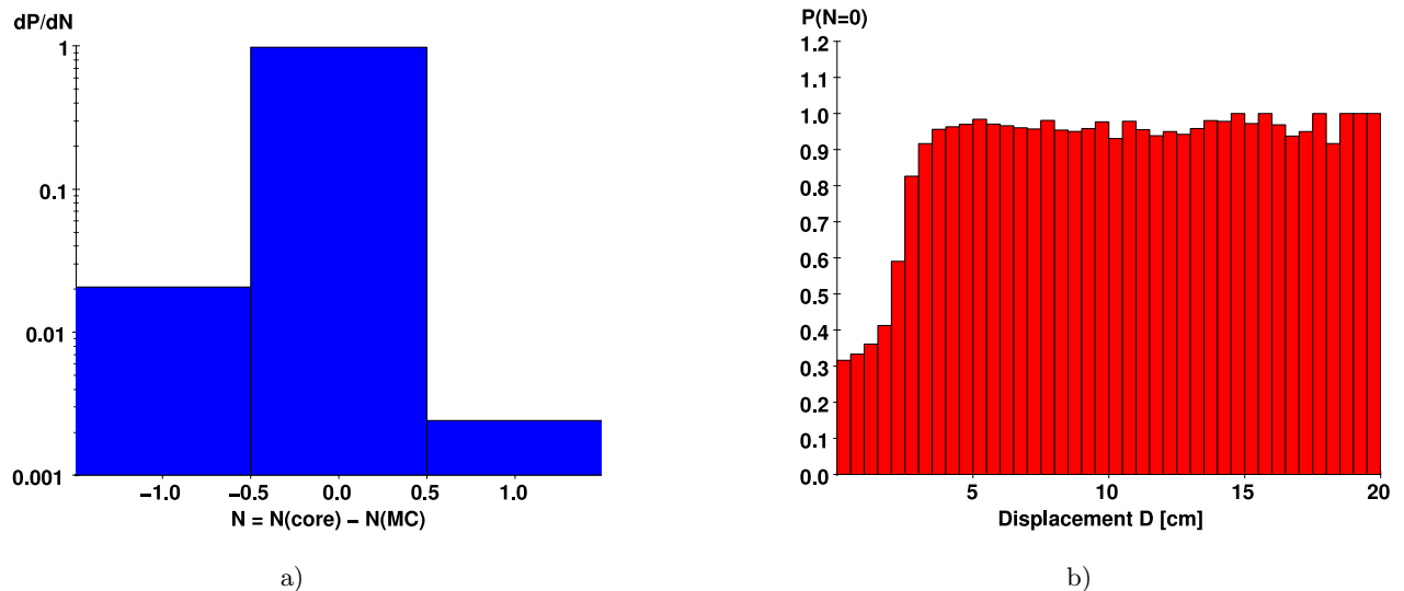
Figure 1: Part a) shows the probability for the number difference N of identified shower cores N(\text{core}) and MC particles N(\text{MC}) for isolated photons, note the logarithmic scale. One shower core per photon, equivalent to N = 0 , is found with about 98 % probability. Part b) shows this probability for photons from K_s^0 \rightarrow \pi^0 \pi^0 decays as a function of the photon displacement D on the calorimeter surface. Significant amounts of merged shower cores are only observed for D < 3 cm.
