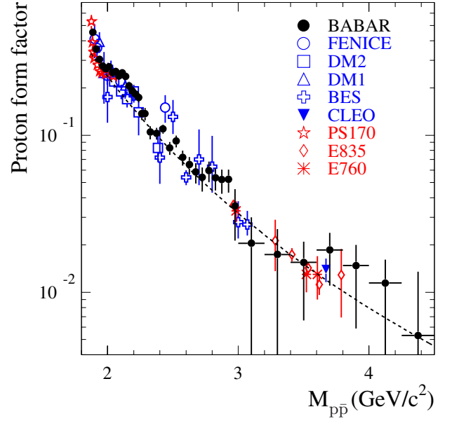
FIG. 19: The proton effective form factor measured in this work and in e^+e^- and p\bar{p} experiments, shown on a logarithmic scale: FENICE[6], DM2[5], DM1[4], BES[8], CLEO[9], PS170[10], E835[12], E760[11]. The curve corresponds to the QCD fit described in the text.
