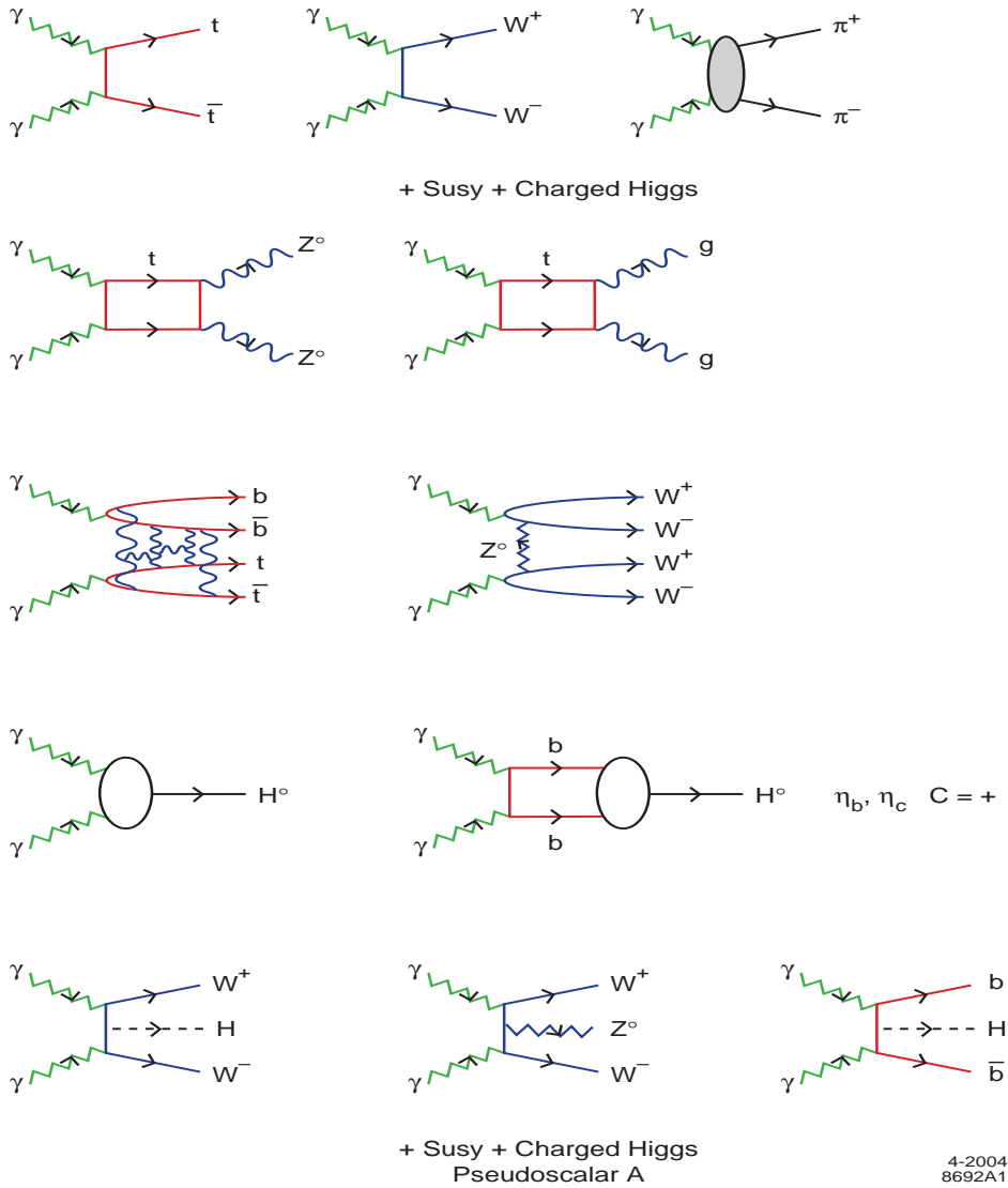
Figure 1: Representative \gamma\gamma processes accessible at a high energy photon-photon collider.
