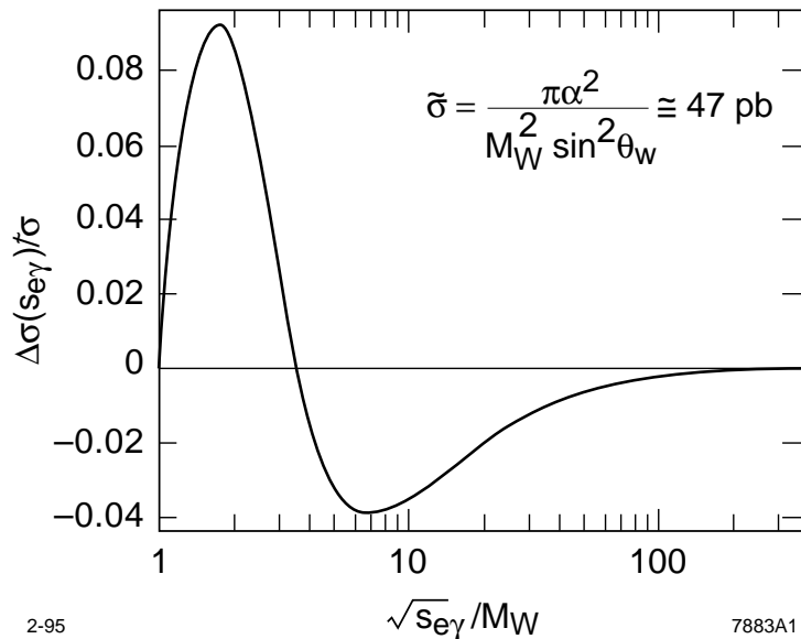
Figure 3: The Born cross section difference \Delta\sigma for the Standard Model process \gamma e \rightarrow W\nu for parallel minus antiparallel electron/photon helicities as a function of \log \sqrt{s_{e\gamma}}/M_W . The logarithmic integral of \Delta\sigma vanishes in the classical limit [49].
