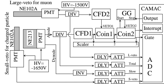
Fig. 2. Electronic measurement circuit. PMT: photo multiplier, CFD: constant fraction discriminator, COIN: coincidence, GG: gate & delay generator, DIV: signal divider, INV: inverter, DLY: delay, ATT: attenuator, ADC: analog to digital converter.
