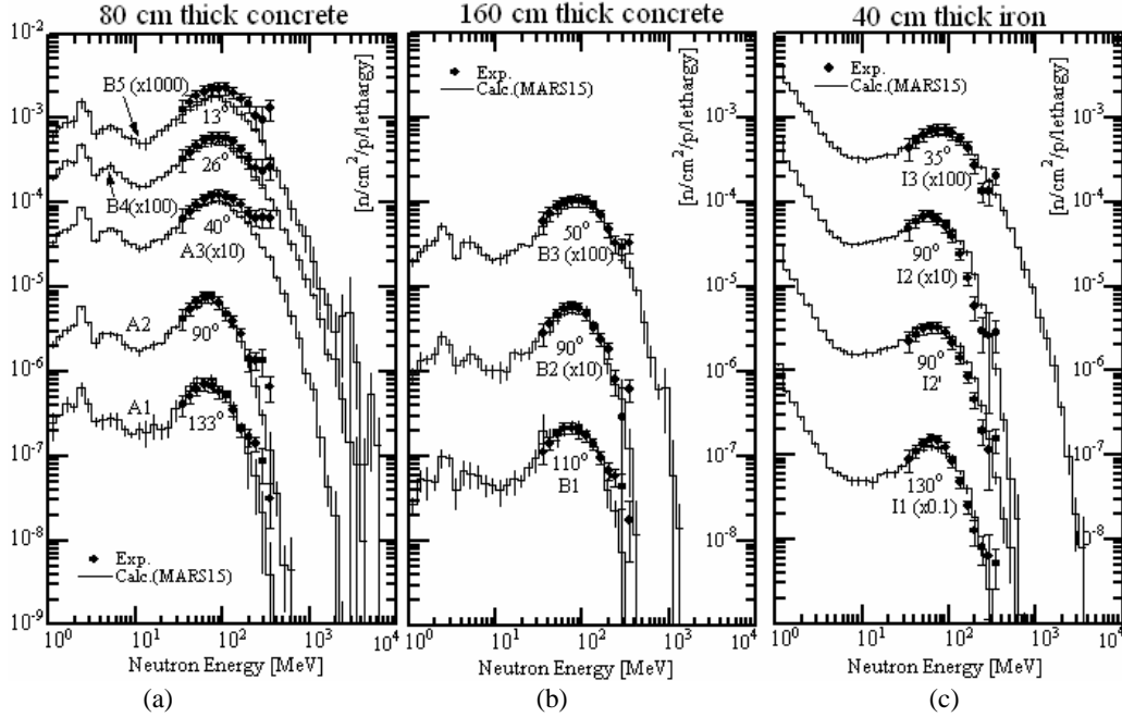
Fig. 3. Experimental neutron energy spectra compared with the MARS15 Monte Carlo calculation results. (a) behind 80-cm thick concrete, (b) behind 160-cm thick concrete and (c) behind 40-cm thick iron.
