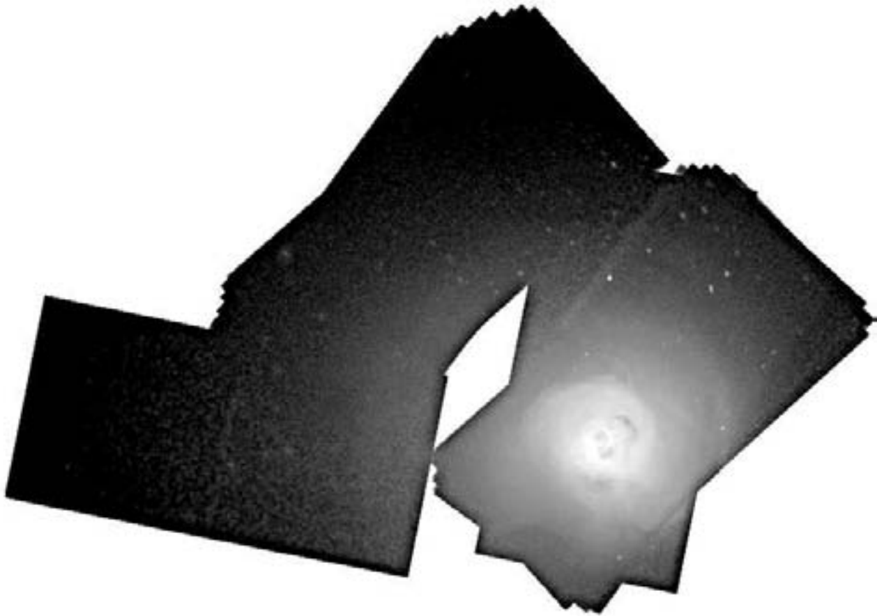
Figure 14. Total image from all Chandra CCD chips.
