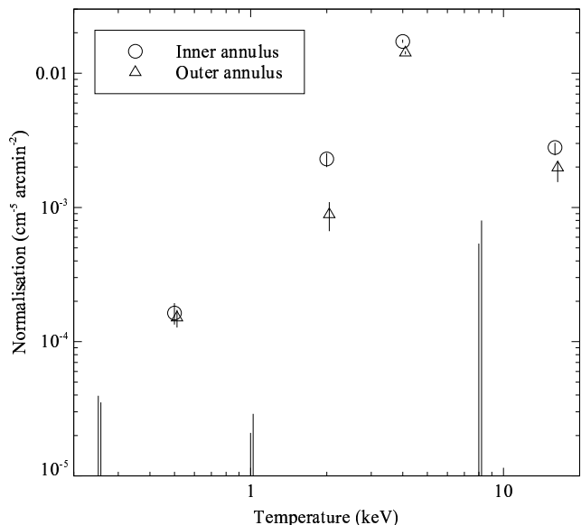
Figure 10. Distribution of temperature components within and outside the shock. Note that both the 4 and 2 keV components increase within the shock, with the 2 keV one increasing proportionately more.
