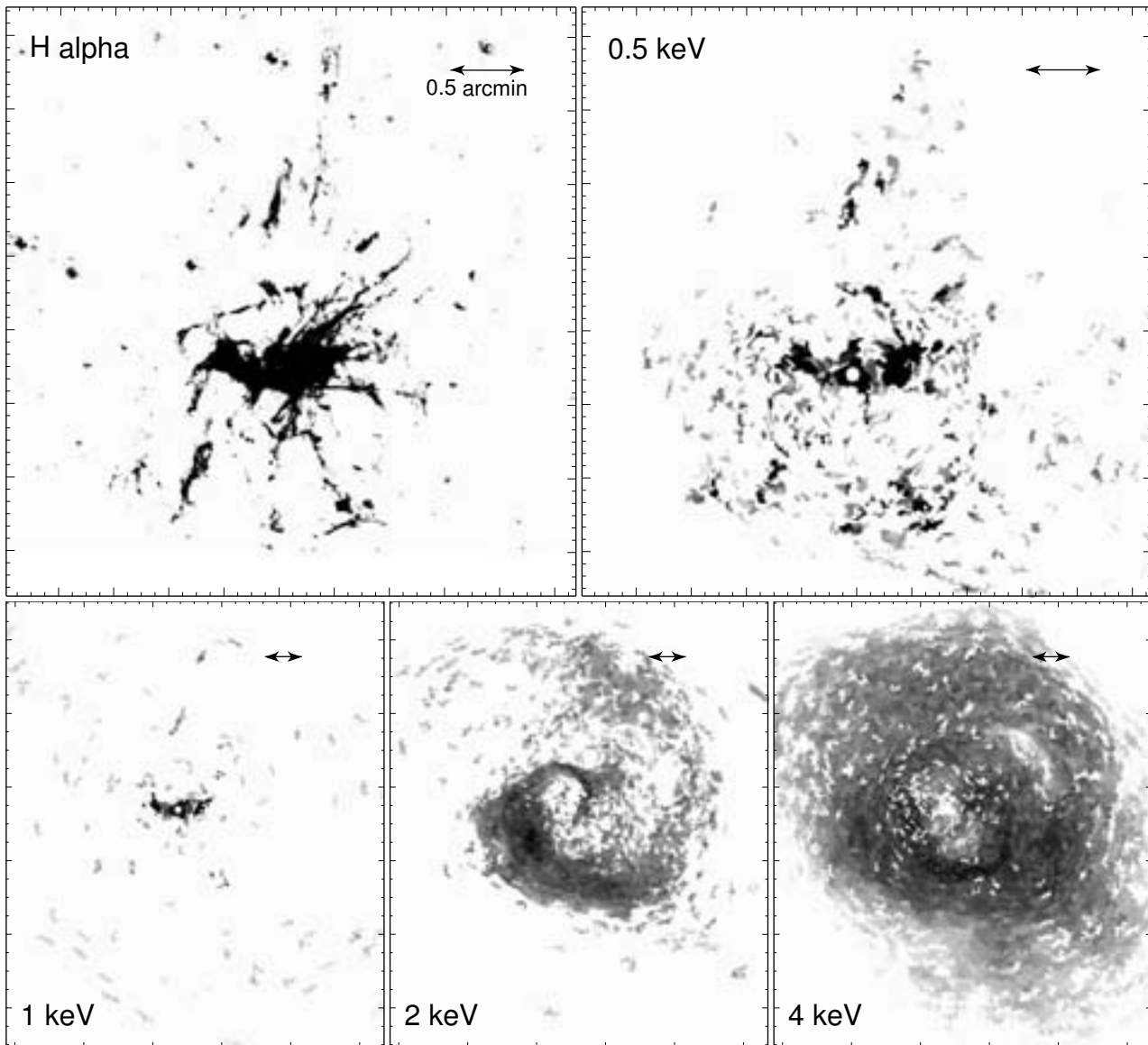
Figure 12. The H\alpha filaments from the optical narrow-band image of Conselice et al (2000) is shown for comparison with maps of the 0.5, 1, 2 and 4 keV components.
