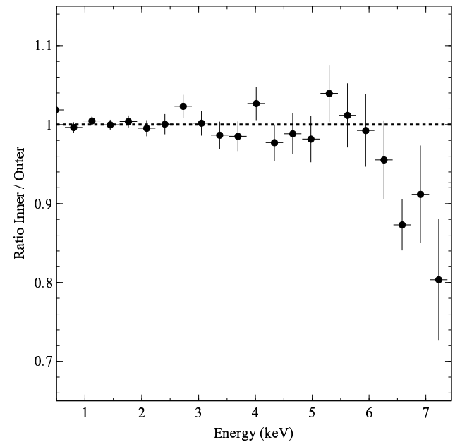
Figure 9. Ratio of the spectrum inside the shock to that outside.
