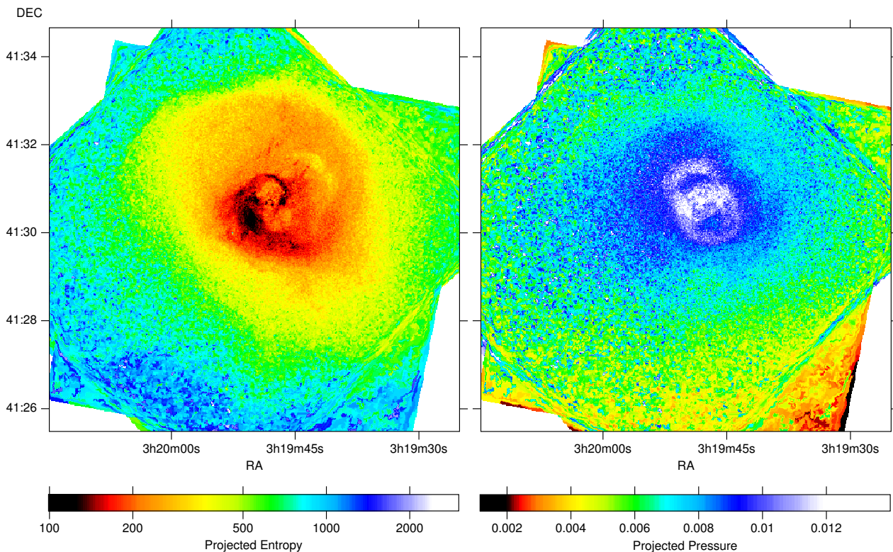
Figure 5. Entropy (left) and pressure (right) maps. The entropy map was calculated using kTA^{-1/3} , in units of \text{keV cm}^{5/3} \text{arcsec}^{2/3} , where A is the MEKAL normalisation per square arcsecond. The pressure map was calculated using kTA^{1/2} , in units of \text{keV cm}^{-5/2} \text{arcsec}^{-1} . These maps were generated by fitting regions containing approximately 625 counts or greater.
