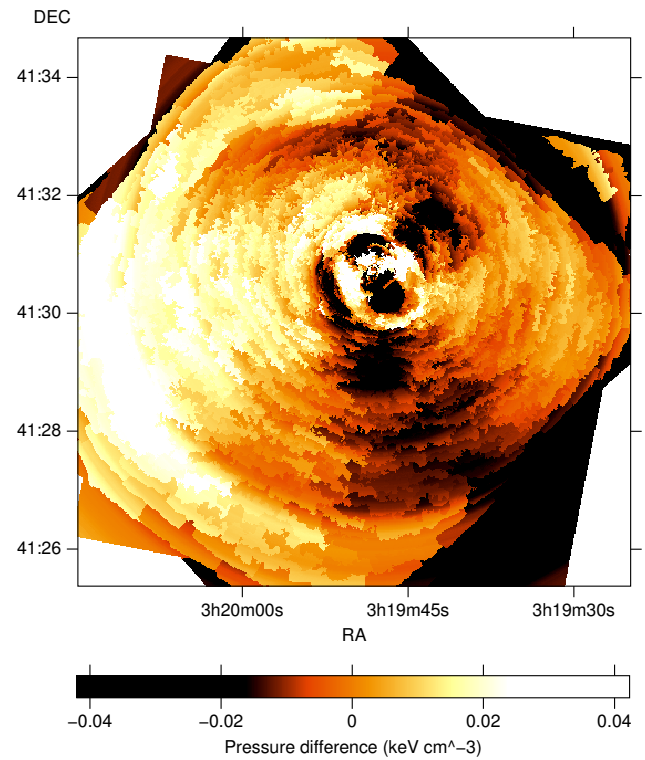
Figure 7. Pressure map where the mean pressure at each radius has been subtracted. In this map the temperatures and normalisations were measured using regions containing approximately 10^4 counts or greater.
