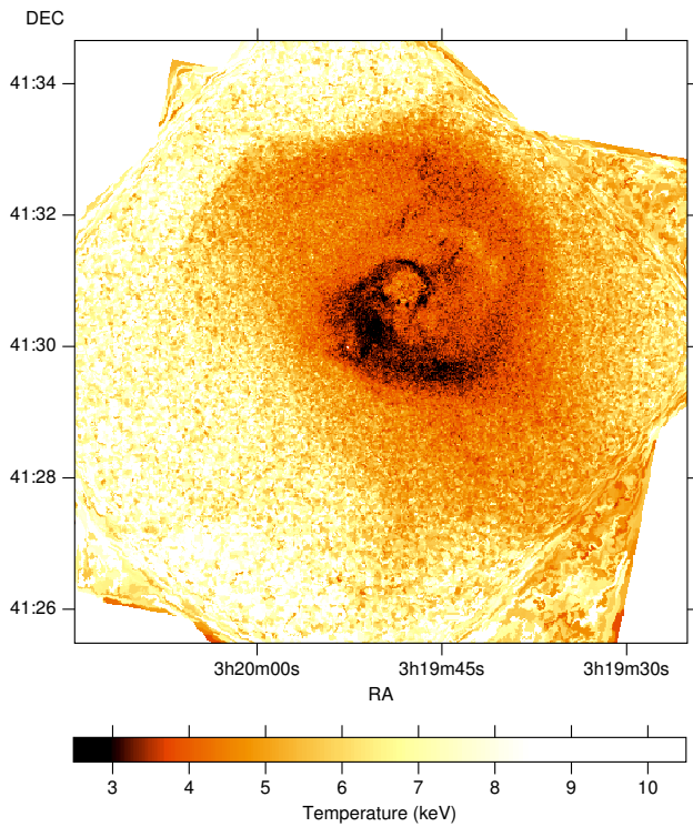
Figure 4. Temperature map calculated by fitting spectra with approximately 625 counts or greater. The uncertainties of the individual fits range from 8 per cent in the coolest regions to 20 per cent in the hottest parts, ignoring the uncertainty on the metallicity and absorbing column density.
