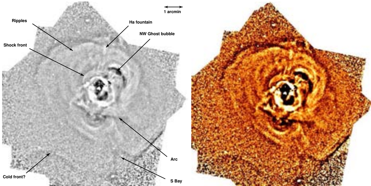
Figure 2. Unsharp mask image made from the whole 0.3–7 keV band by subtracting an image smoothed with a Gaussian of dispersion 10 arcsec from one smoothed by 1 arcsec. Various features are labelled on the lower contrast image at the left.
