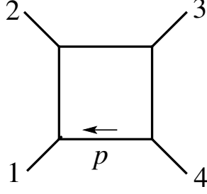
FIG. 6: The one-loop box integral.
