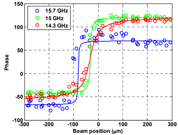
Figure 4: Signal phase as a function of beam position.
