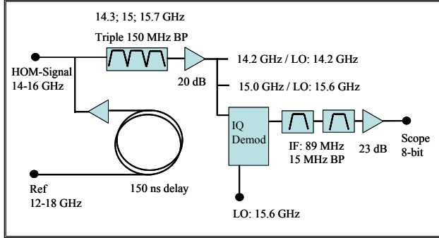
Figure 2: Schematics of the signal processing electronics
