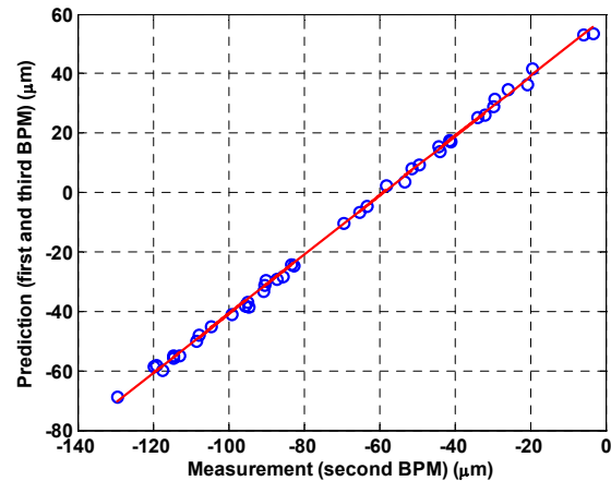
Figure 5: Prediction versus measurement for the middle BPM of the accelerating structure.
