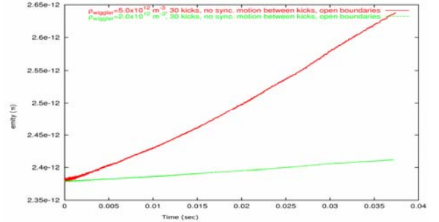
Figure 5. Evolution of the vertical emittance for different electron cloud density assuming the electron cloud occurs only in the 540m long wiggler sections of the 17 km DR.
