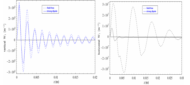
Figure 7. (Left) Vertical and (Right) Horizontal wake fields computed for the DR 17 km in field free and strong dipole field. Cloud size (10,10) in units of (\sigma_x, \sigma_y) and cloud density \rho_e = 10^{12} \text{ m}^{-3} .
