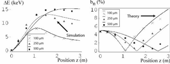
Figure 2- a-b Energy modulation / Current modulation for a 12 MeV beam along a drift; comparison with theory for single and multiple frequency
