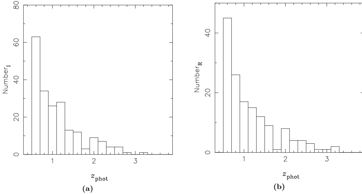
Fig. 4. The redshift distributions of background sources used for weak lensing analysis (only sources with z_{\text{phot}} > 0.55 were considered) for I-band a) and R-band catalogue b) . The mean photometric redshift of the samples is \langle z_I \rangle = 1.18 and \langle z_R \rangle = 1.14 .
