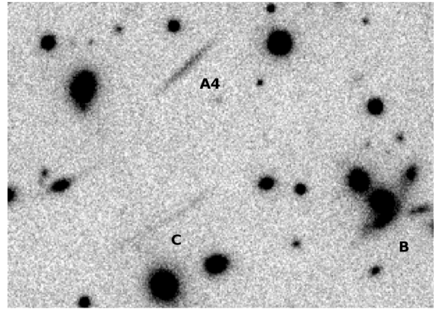
Fig. 8. A \sim 1'.0 \times 0'.6 cutout of the Ks-band image of RX J1347.5–1145 showing one of the arcs used for strong lensing, the newly discovered very red arc system B1-B2 (two images almost merging, c.f. Fig. 6) and the long thin arc C.
