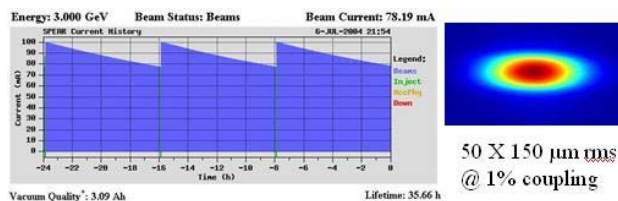
Figure 6: Typical SPEAR 3 operation with 8-h fills (left) and X-ray pinhole camera beam image (right).
