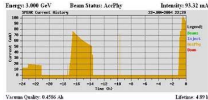
Figure 2: First 100-mA, 1/22/04.
