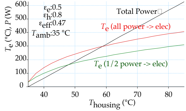
Figure 4: Electrode temperature.
