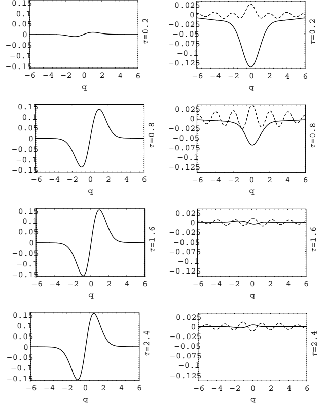
Figure 2: Dimensionless wake force IF(q) (in notation of [3]) proportional to (12), at successive times. First term on left graph, second (solid) and third (dashed) on right. q = (\theta - \omega_0 t)R / \sigma_z , \sigma_z = bunch length.
